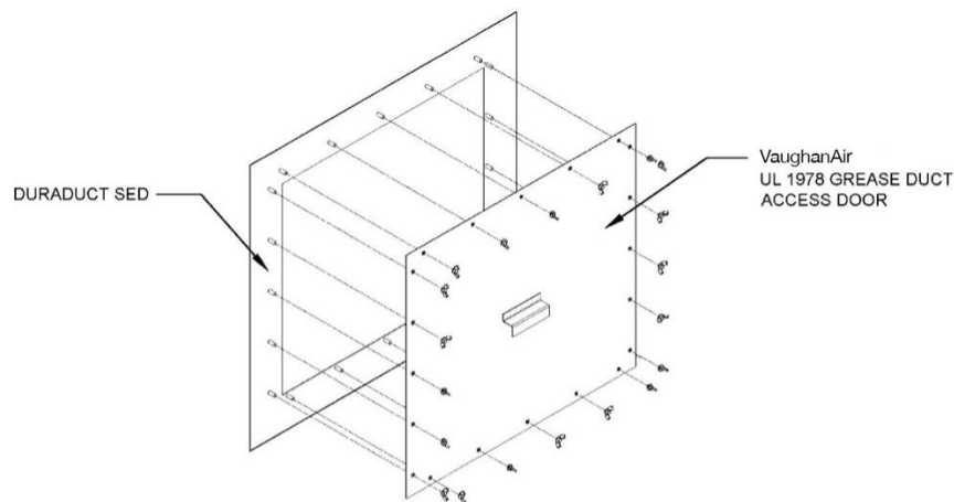
Access Panel Detail
