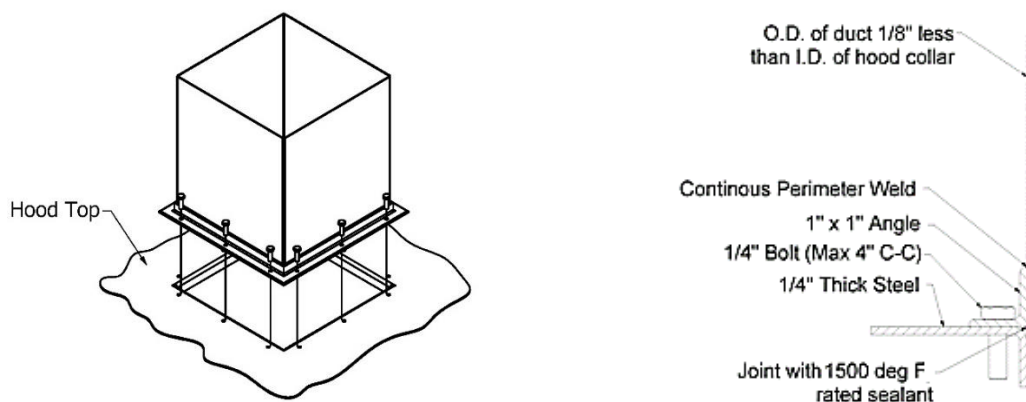
Non-Weld Hood Connection Details
