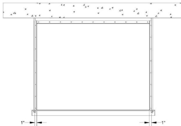
Cradle/Rod Location Detail
