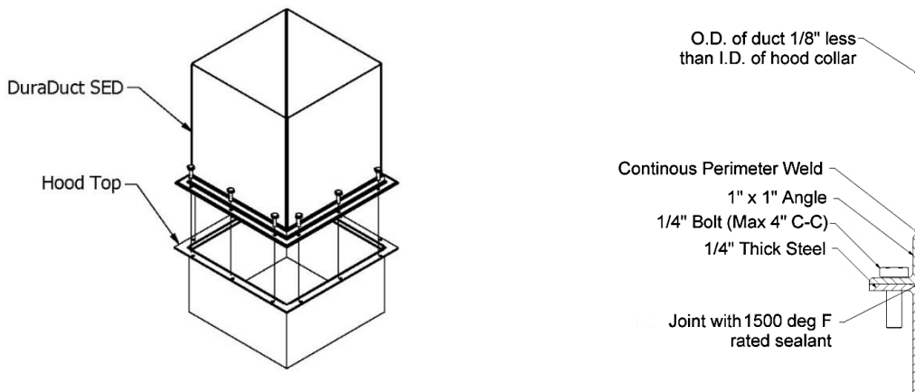
Non-Weld Hood Connection Details
